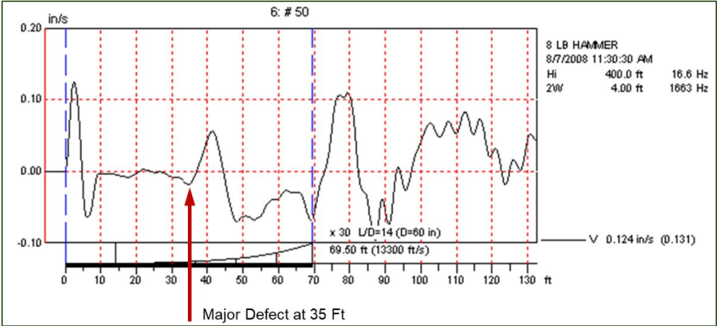
Figure 26. Representative pulse echo low strain integrity test record with reflection from a major defect.
